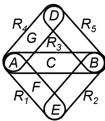
Figure 2.2: Hypergraph.
