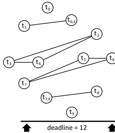
Figure 5.9: Graph for unsolvable CS identification
