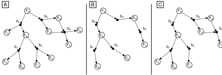
Figure 4.10: (A) BFG for the graph in Figure 4.6 - (B) the s -tree associated to the scenario \neg a \neg b \neg c \neg d e - (C) a subgraph (set of s -trees) associated to scenarios where \neg ace holds
