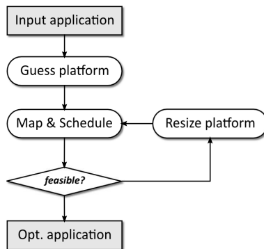
Figure 2.3: Basic design space exploration algorithm
