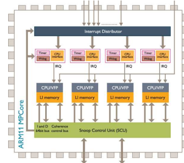
Figure 2.2: Block diagram for the ARM11 MPCore processor
